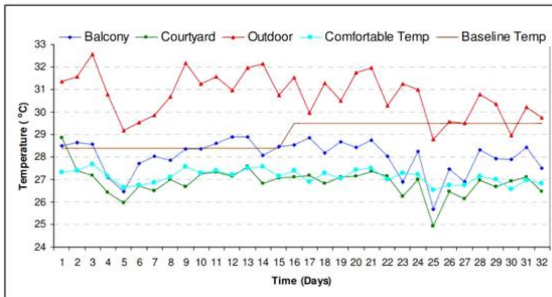
Fig. 4: Comparison between the houses with comfortable and baseline temperatures
