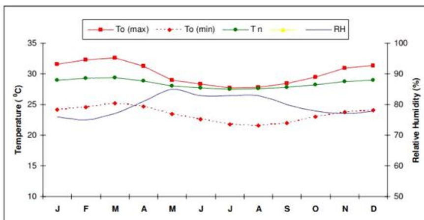
Figure 1: Monthly neutral temperature variations in relation to mean maximum and mean minimum and relative humidity of a typical year of Mombasa
