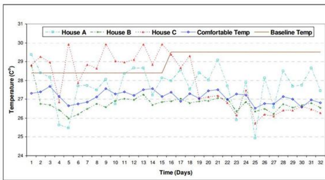
Figure 4: Comparison between the houses with comfortable and baseline temperatures
