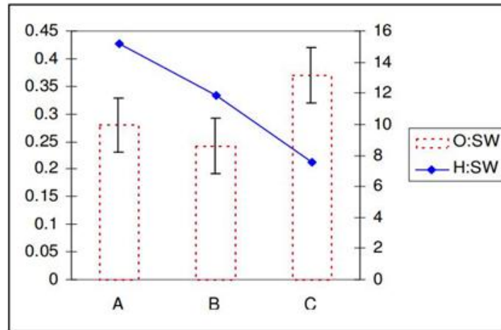
Figure 3: Openings to solid wall surface area ratio and building height to street width ratio
