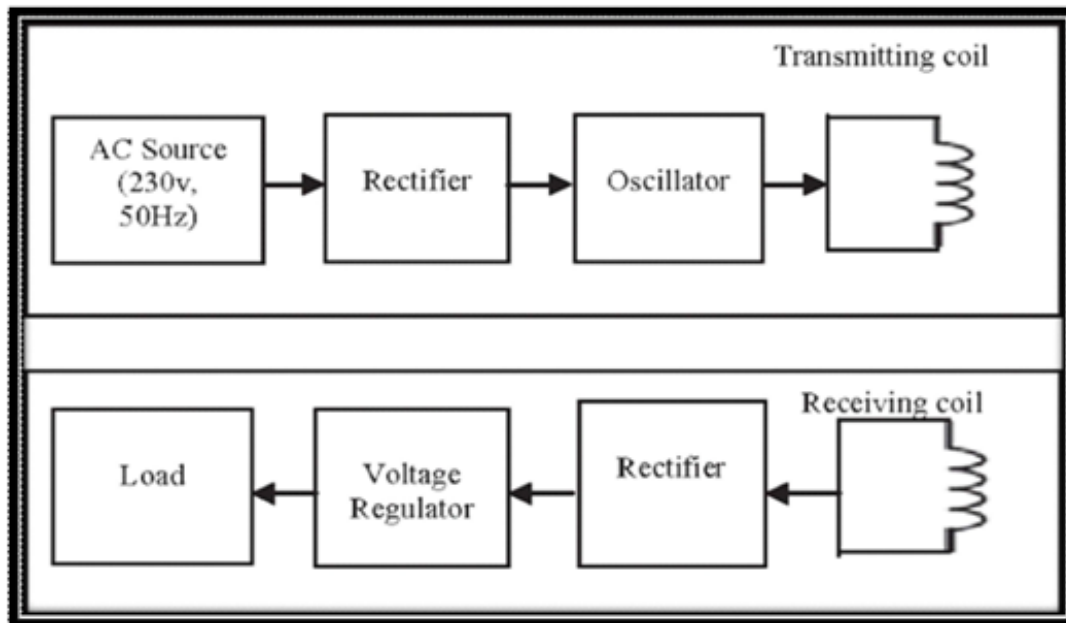
Fig.1: Block Diagram of Wireless Power Transfer System
